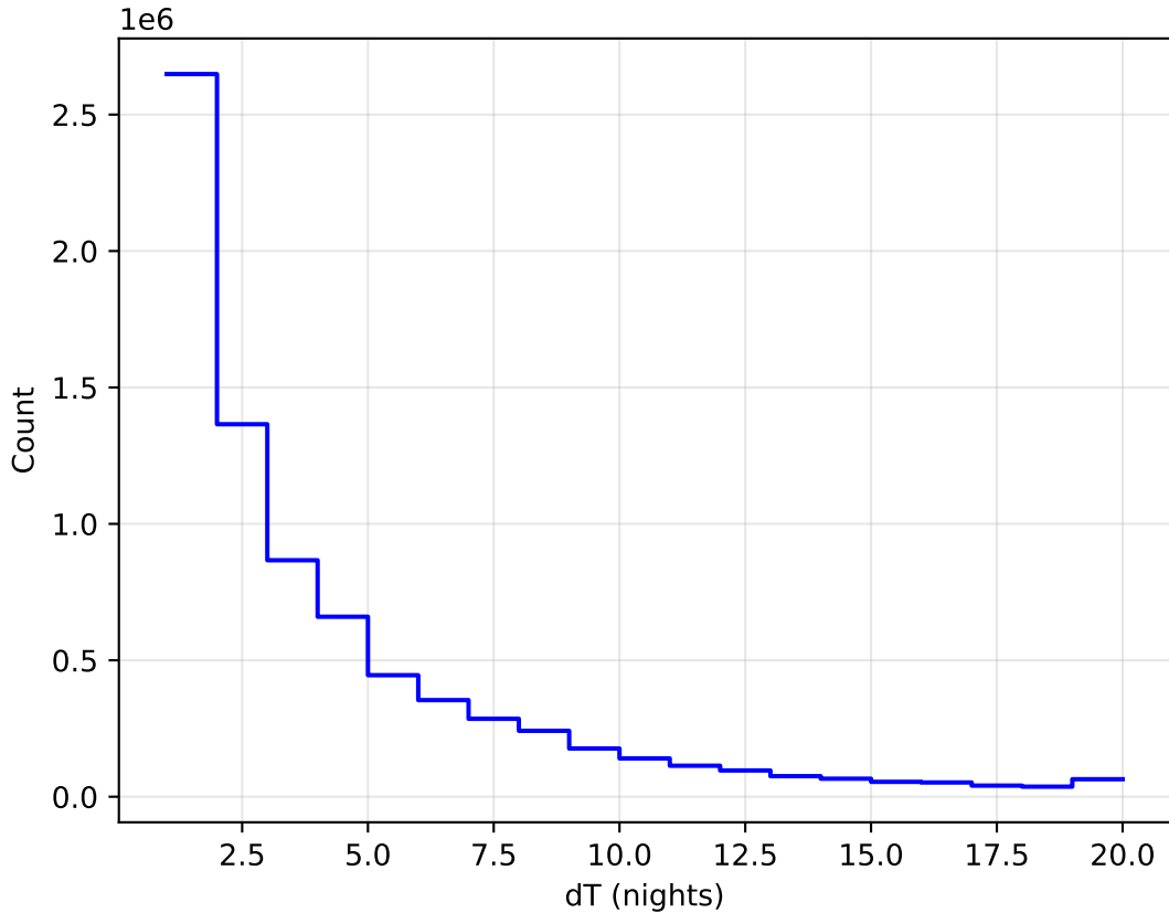
ddf_acor_sf25_lsf30_lsr10_v3.4_10yrs WFD all bands: DeltaNight Histogram
