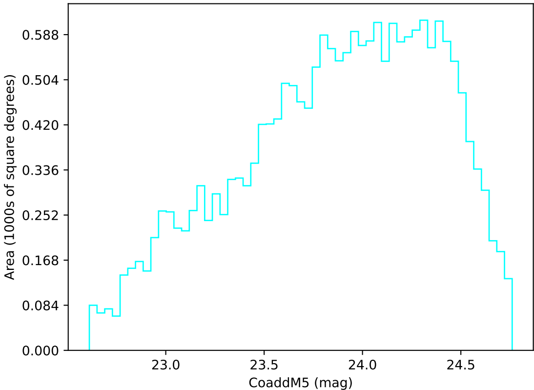
ddf_acor_sf25_lsf30_lsr10_v3.4_10yrs Yr 3-4 u band: CoaddM5
