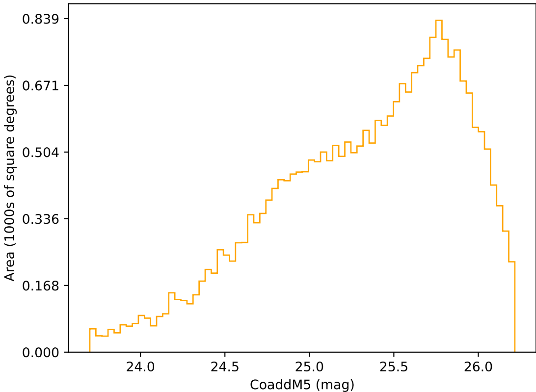
ddf_acor_sf25_lsf30_lsr10_v3.4_10yrs Yr 3-4 r band: CoaddM5
