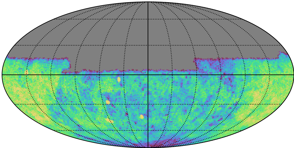
ddf_acor_sf25_lsf30_lsr10_v3.4_10yrs Yr 1 u band: CoaddM5
