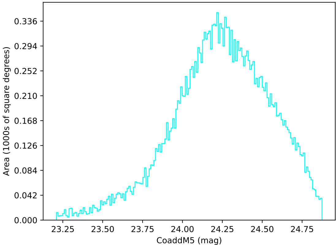
ddf_acor_sf25_lsf30_lsr10_v3.4_10yrs Yr 1 u band: CoaddM5
