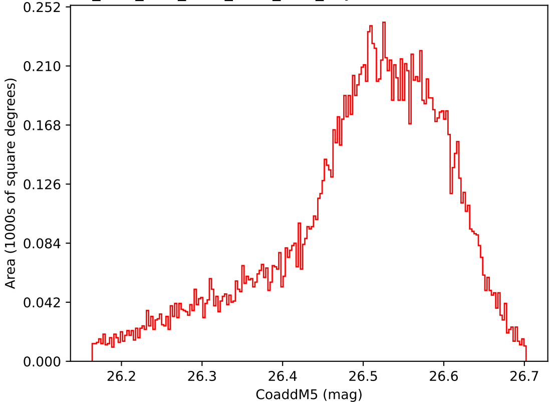
ddf_acor_sf25_lsf30_lsr10_v3.4_10yrs WFD i band: CoaddM5
