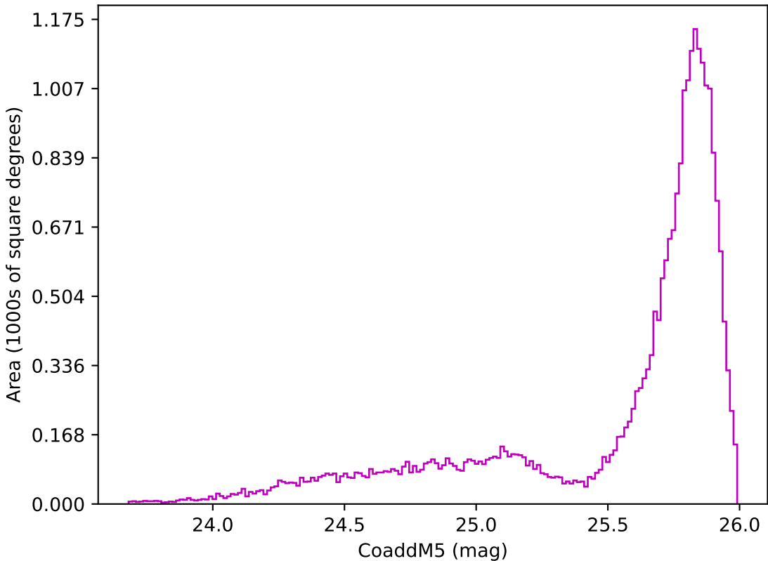
ddf_acor_sf25_lsf30_lsr10_v3.4_10yrs All sky z band: CoaddM5
