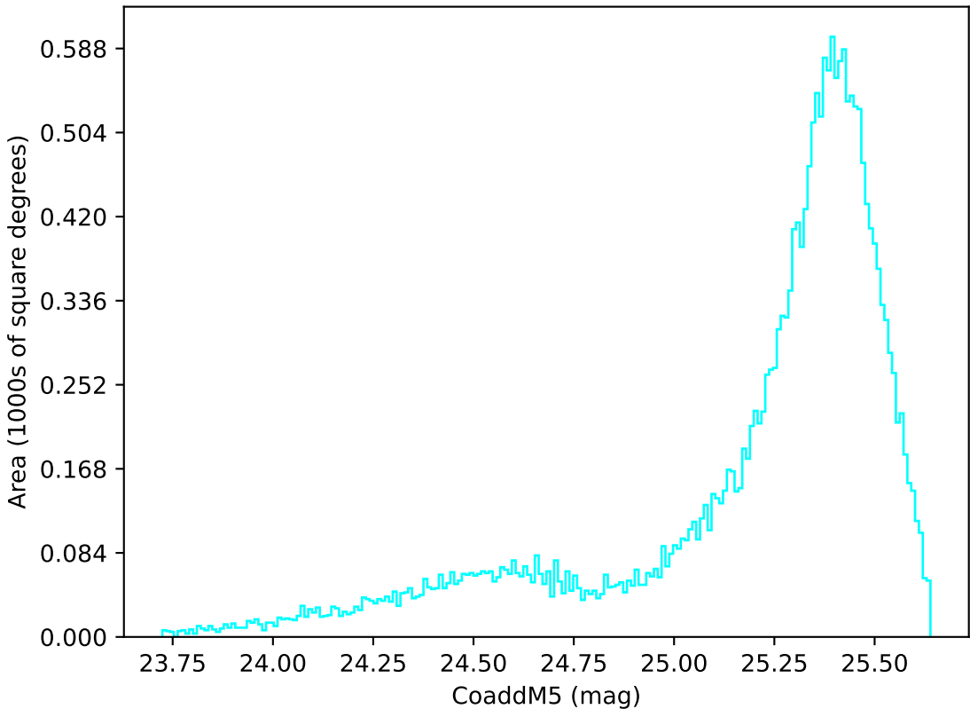
ddf_acor_sf25_lsf30_lsr10_v3.4_10yrs All sky u band: CoaddM5
