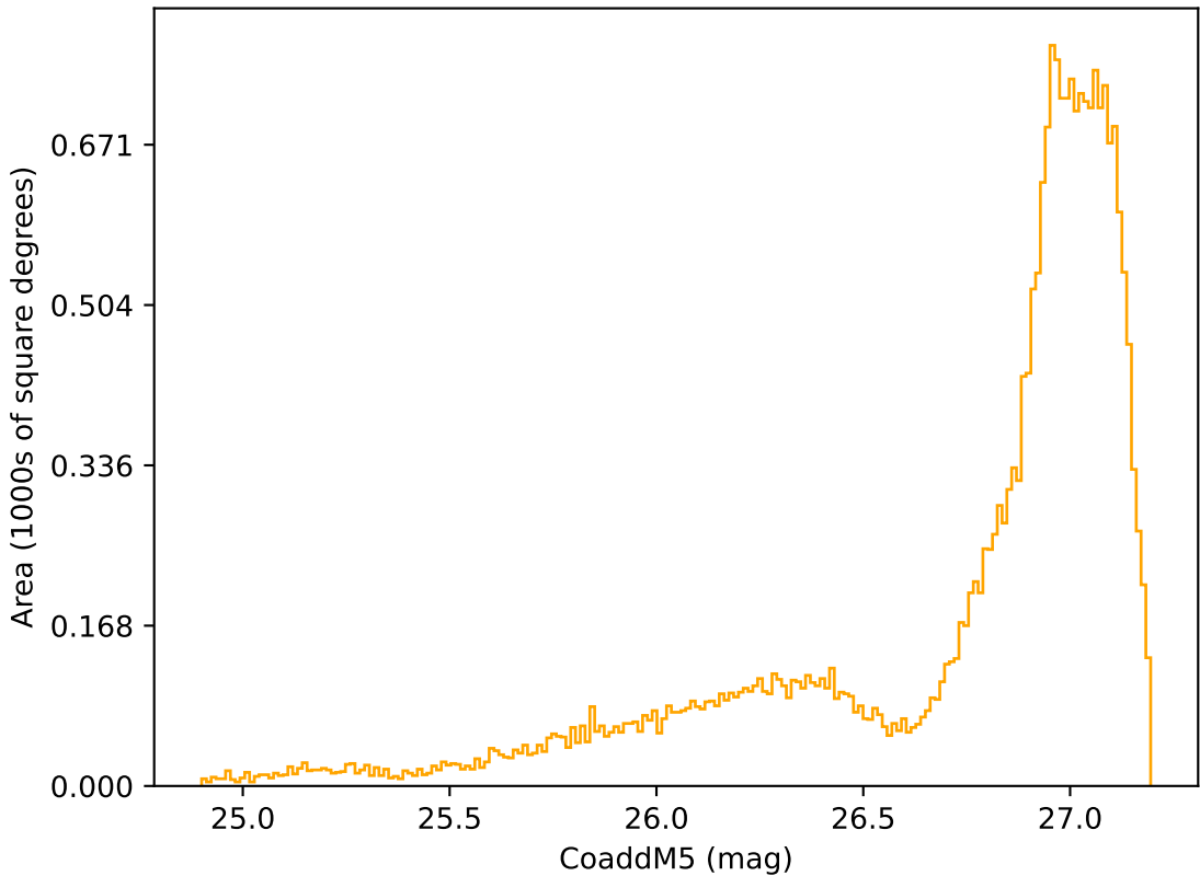
ddf_acor_sf25_lsf30_lsr10_v3.4_10yrs All sky r band: CoaddM5
