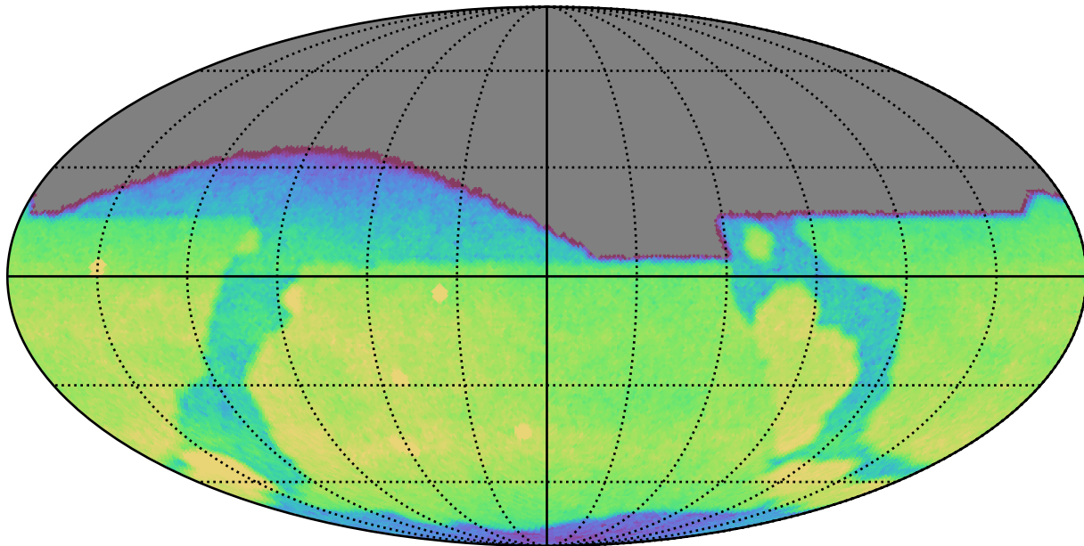
ddf_acor_sf25_lsf30_lsr10_v3.4_10yrs All sky g band: CoaddM5
