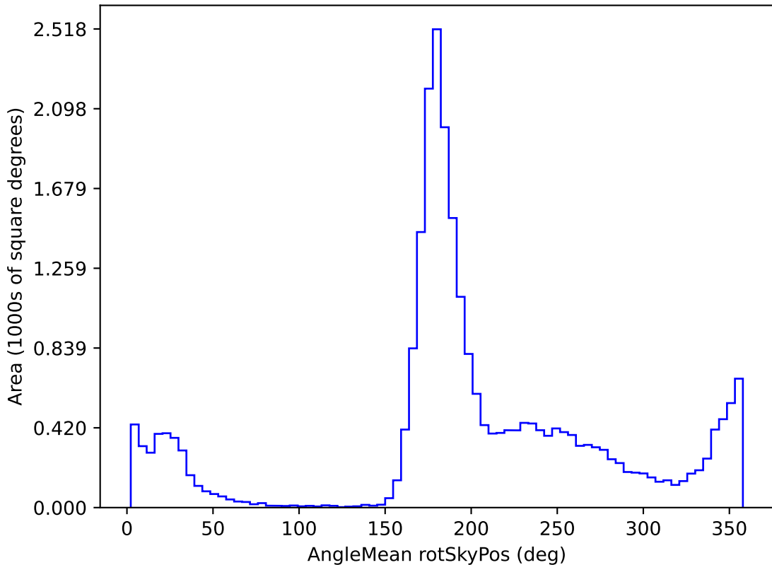
ddf_acor_sf25_lsf30_lsr10_v3.4_10yrs All sky r band: AngleMean rotSkyPos
