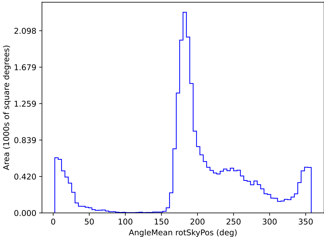
ddf_acor_sf25_lsf30_lsr10_v3.4_10yrs All sky i band: AngleMean rotSkyPos
