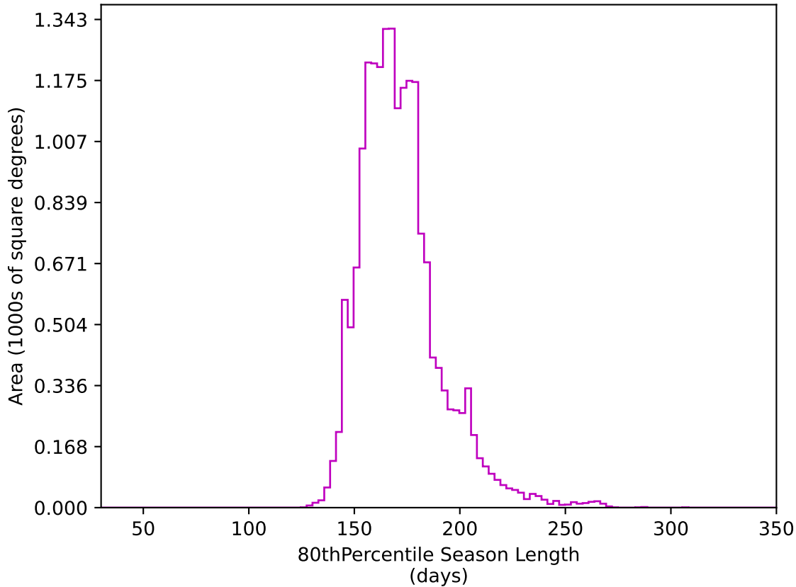
ddf_acor_sf25_lsf30_lsr10_v3.4_10yrs WFD z band: 80thPercentile Season Length
