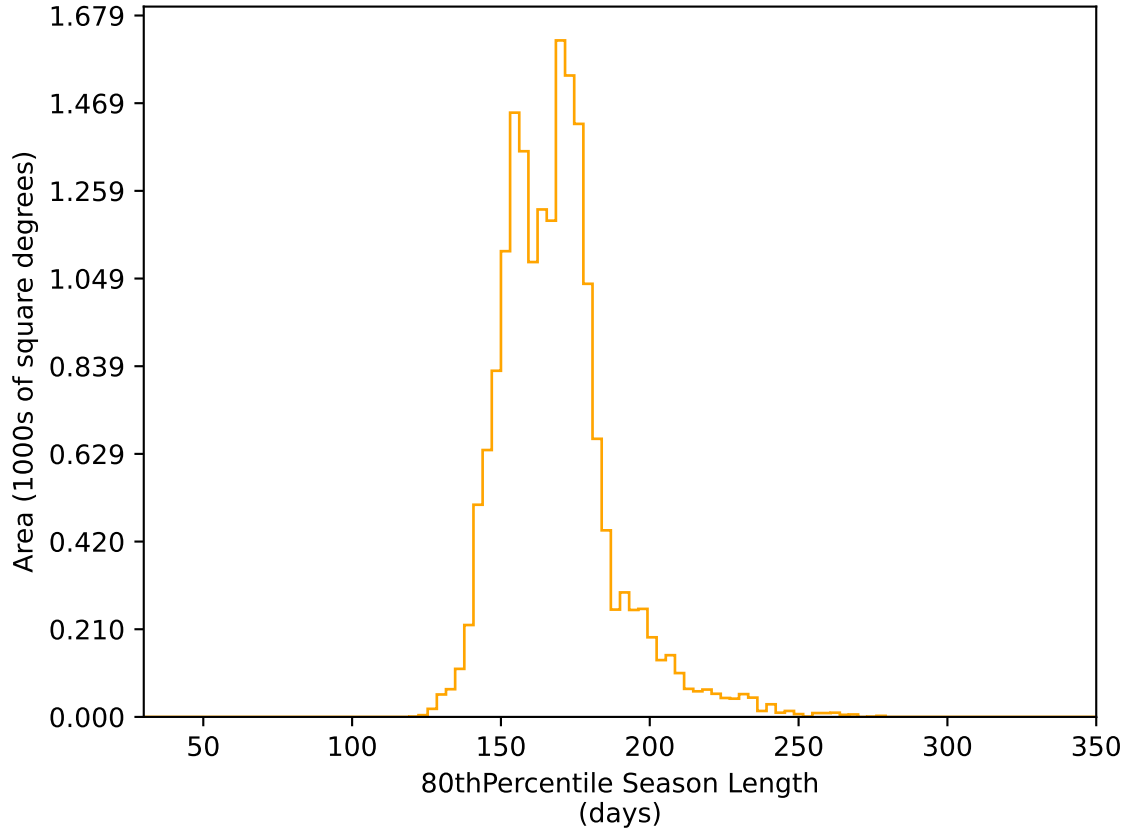
ddf_acor_sf25_lsf30_lsr10_v3.4_10yrs WFD r band: 80thPercentile Season Length
