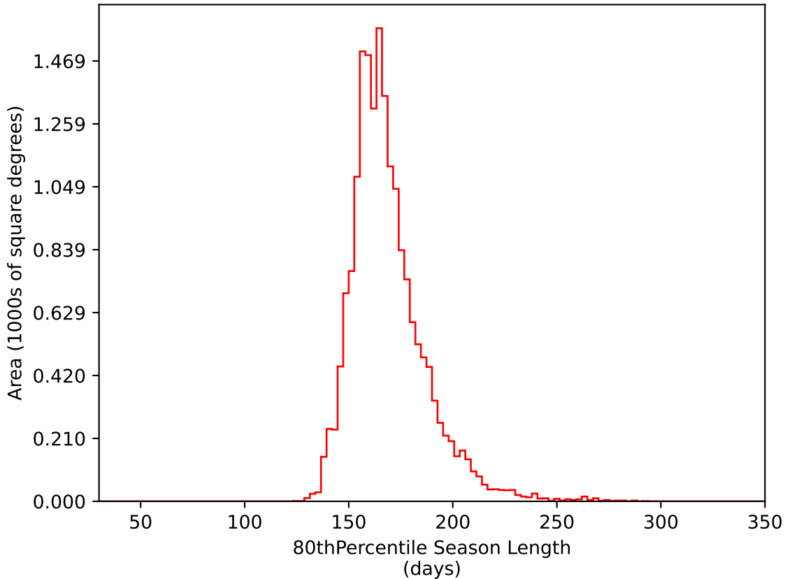
ddf_acor_sf25_lsf30_lsr10_v3.4_10yrs WFD i band: 80thPercentile Season Length
