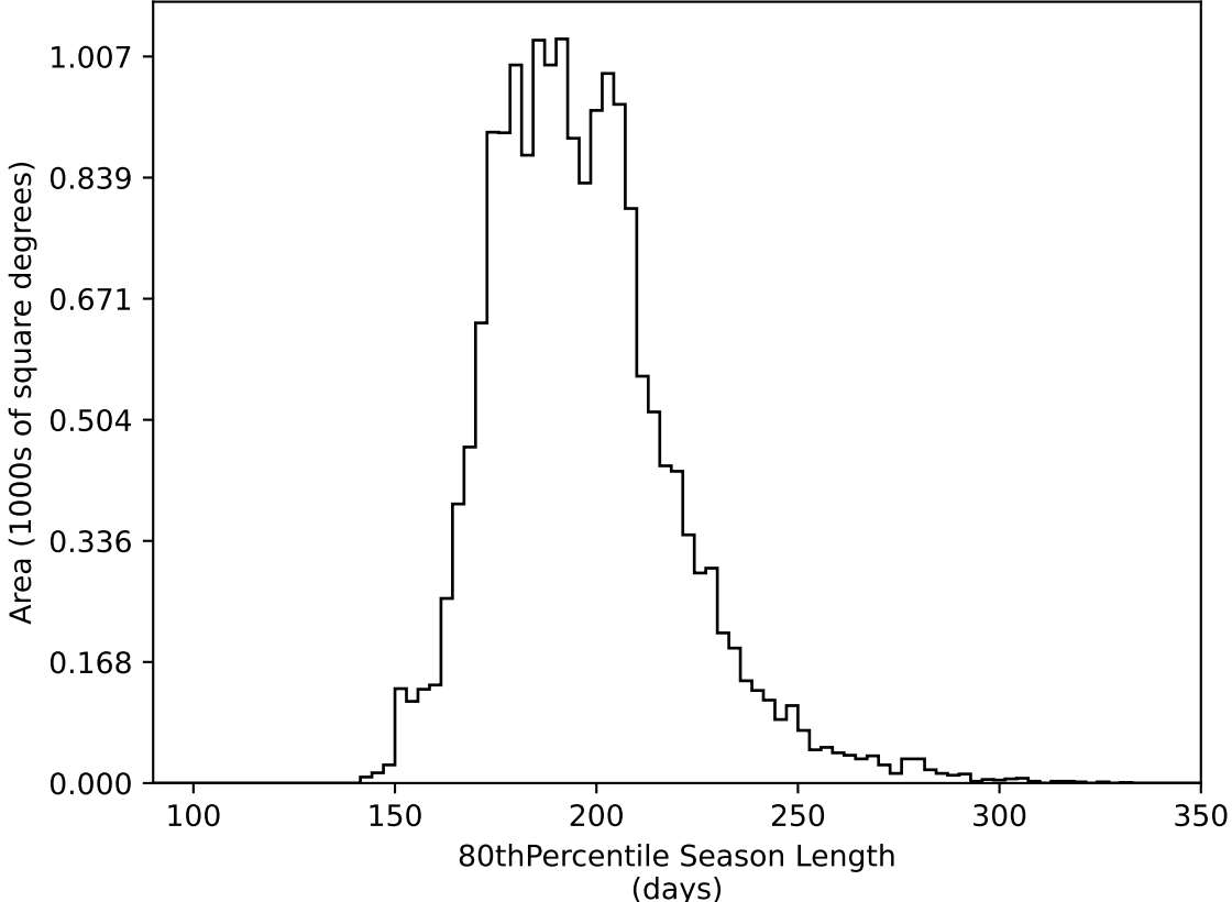
ddf_acor_sf25_lsf30_lsr10_v3.4_10yrs WFD all bands: 80thPercentile Season Length
