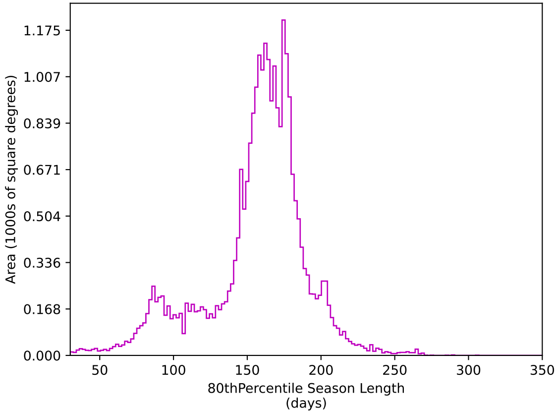
ddf_acor_sf25_lsf30_lsr10_v3.4_10yrs All sky z band: 80thPercentile Season Length
