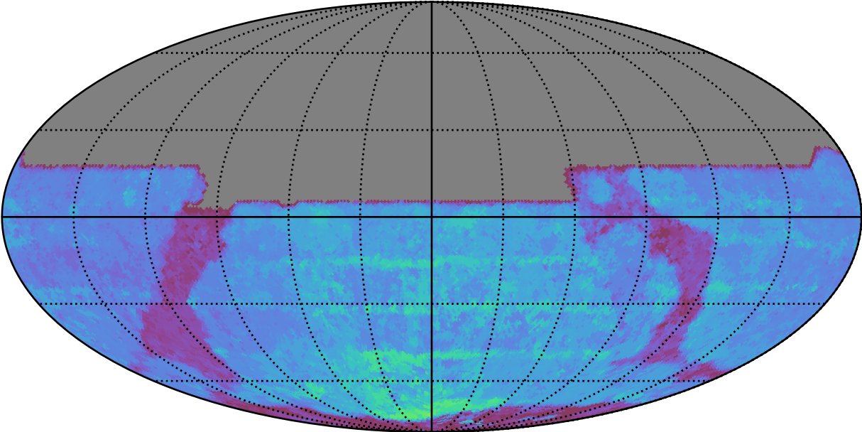
ddf_acor_sf25_lsf30_lsr10_v3.4_10yrs All sky y band: 80thPercentile Season Length
