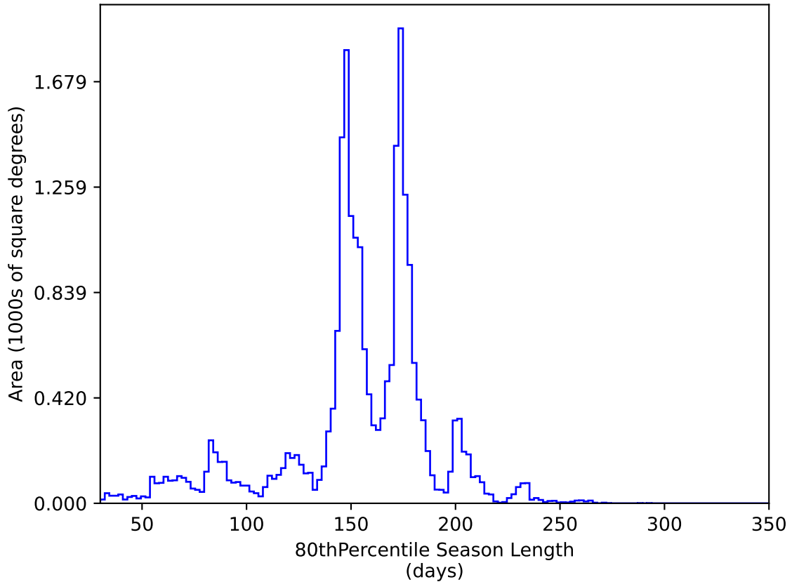
ddf_acor_sf25_lsf30_lsr10_v3.4_10yrs All sky y band: 80thPercentile Season Length
