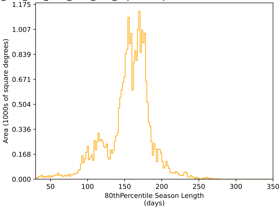
ddf_acor_sf25_lsf30_lsr10_v3.4_10yrs All sky r band: 80thPercentile Season Length
