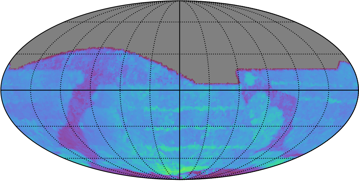
ddf_acor_sf25_lsf30_lsr10_v3.4_10yrs All sky i band: 80thPercentile Season Length
