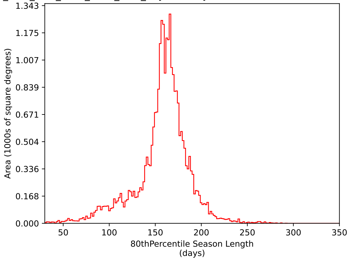
ddf_acor_sf25_lsf30_lsr10_v3.4_10yrs All sky i band: 80thPercentile Season Length
