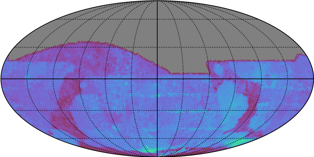
ddf_acor_sf25_lsf30_lsr10_v3.4_10yrs All sky g band: 80thPercentile Season Length
