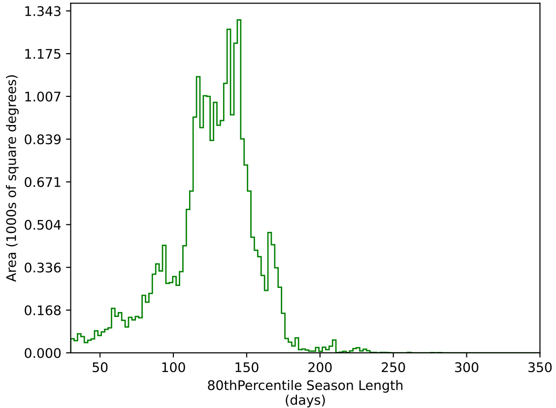
ddf_acor_sf25_lsf30_lsr10_v3.4_10yrs All sky g band: 80thPercentile Season Length
