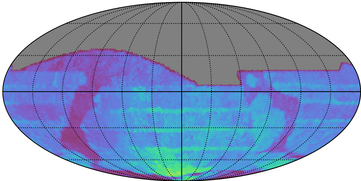
ddf_acor_sf25_lsf30_lsr10_v3.4_10yrs All sky all bands: 80thPercentile Season Length
