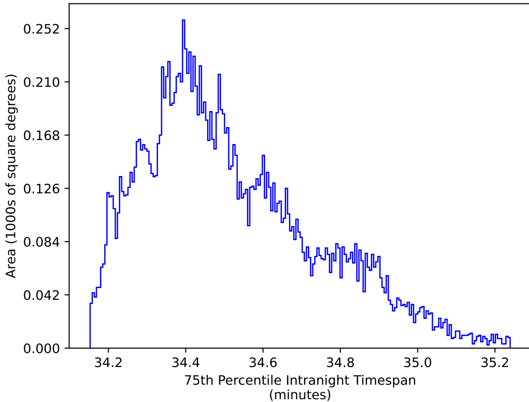
ddf_acor_sf25_lsf30_lsr10_v3.4_10yrs WFD zy bands: 75th Percentile Intranight Timespan
