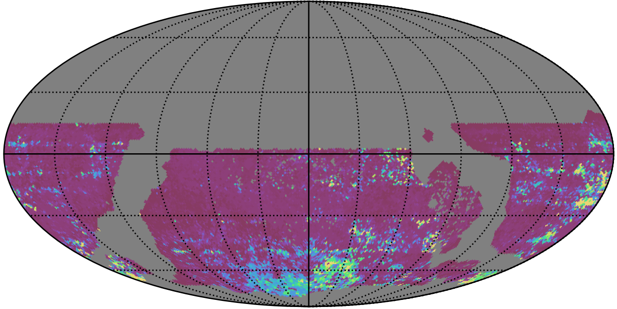
ddf_acor_sf25_lsf30_lsr10_v3.4_10yrs WFD z band: 75th Percentile Intranight Timespan
