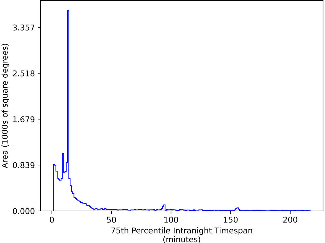
ddf_acor_sf25_lsf30_lsr10_v3.4_10yrs WFD z band: 75th Percentile Intranight Timespan
