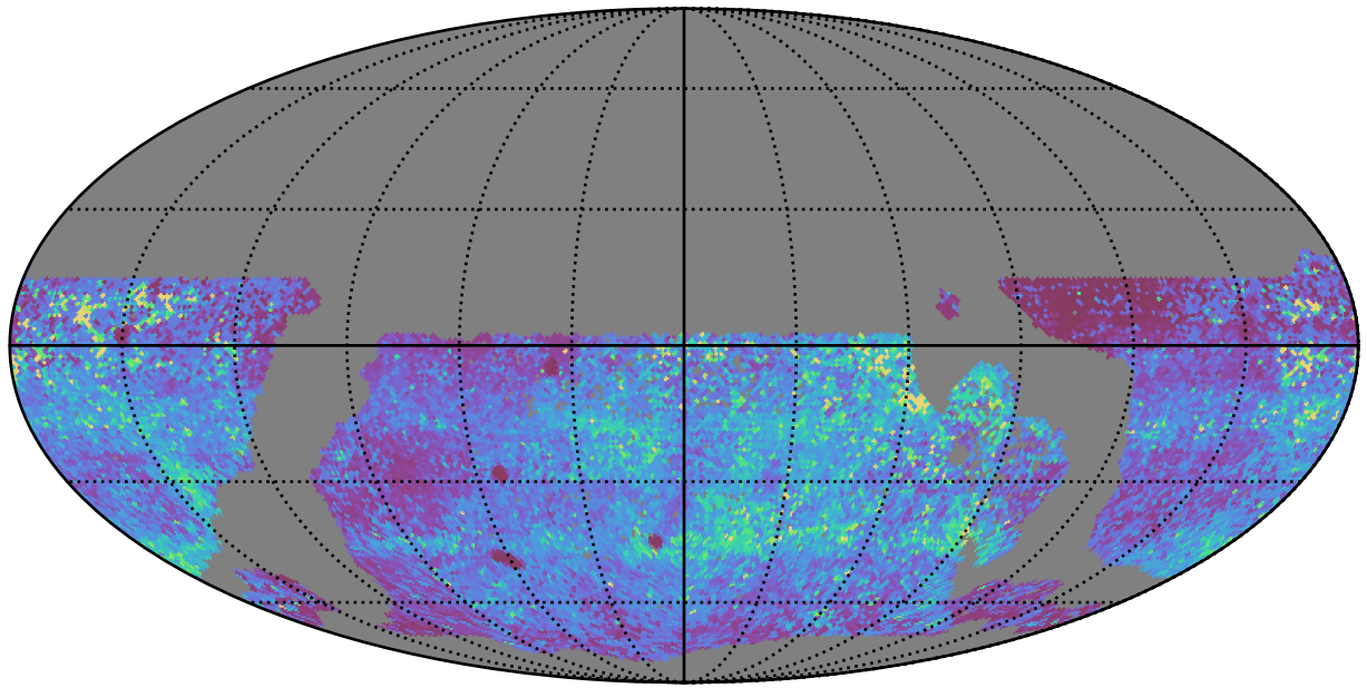
ddf_acor_sf25_lsr10_v3.4_10yrs WFD y band: 75th Percentile Intranight Timespan
