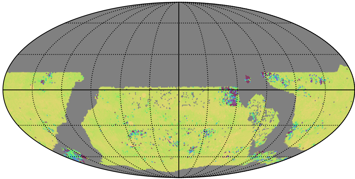
ddf_acor_sf25_lsf30_lsr10_v3.4_10yrs WFD ug bands: 75th Percentile Intranight Timespan
