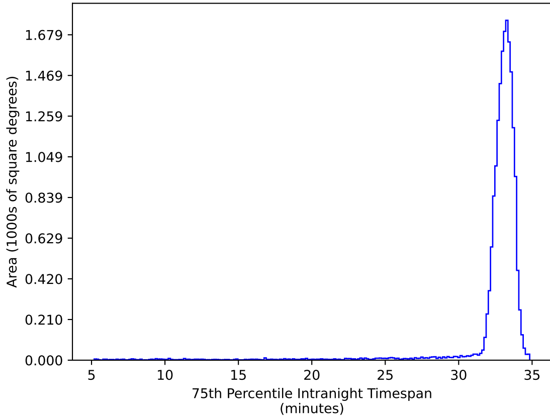
ddf_acor_sf25_lsf30_lsr10_v3.4_10yrs WFD ug bands: 75th Percentile Intranight Timespan
