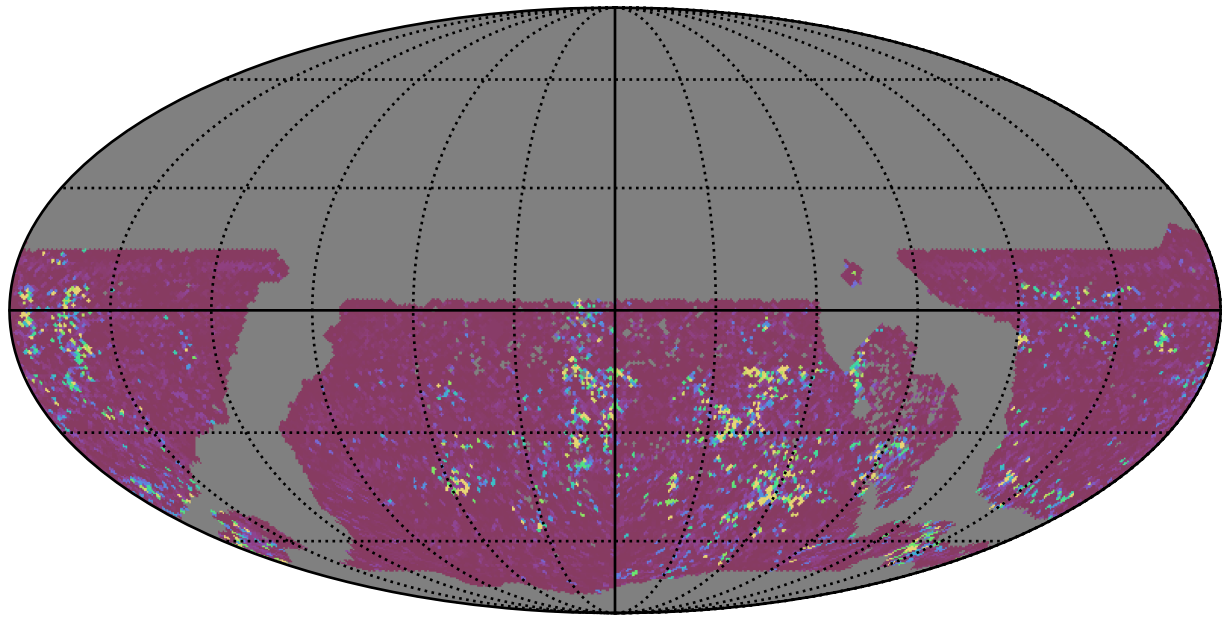
ddf_acor_sf25_lsf30_lsr10_v3.4_10yrs WFD u band: 75th Percentile Intranight Timespan
