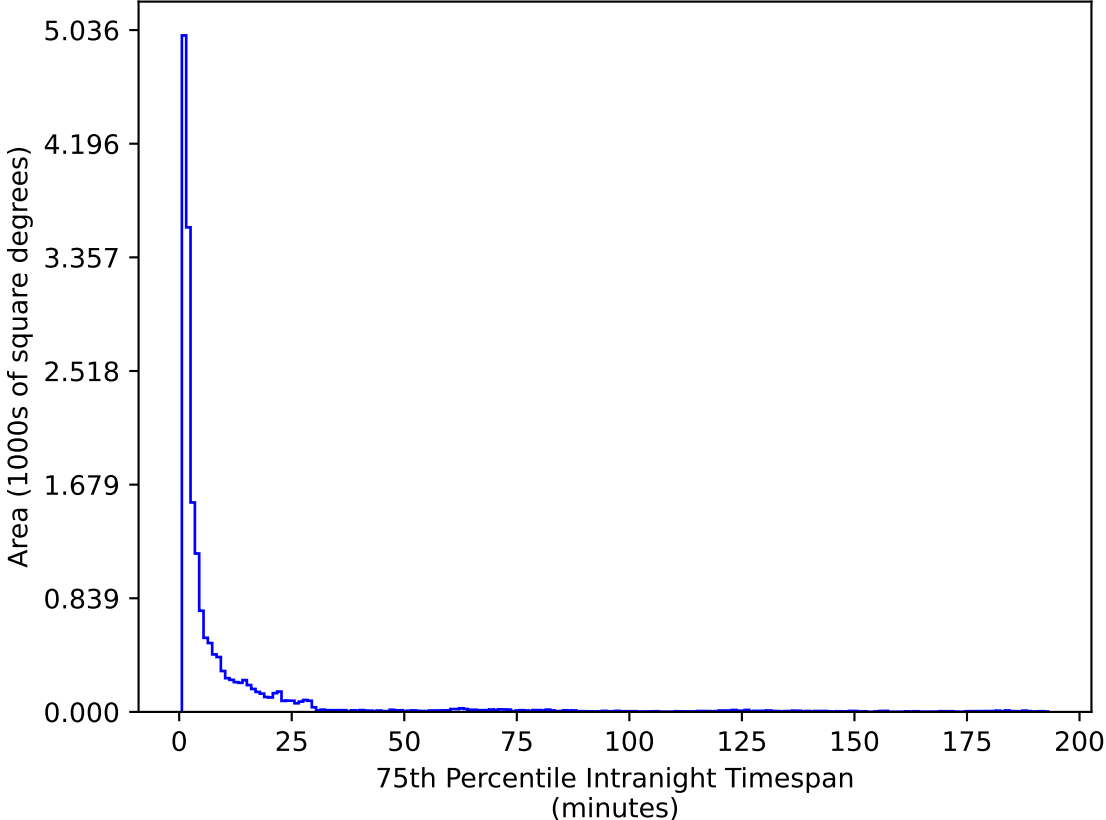
ddf_acor_sf25_lsf30_lsr10_v3.4_10yrs WFD u band: 75th Percentile Intranight Timespan
