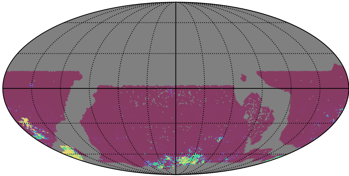
ddf_acor_sf25_lsf30_lsr10_v3.4_10yrs WFD ri bands: 75th Percentile Intranight Timespan
