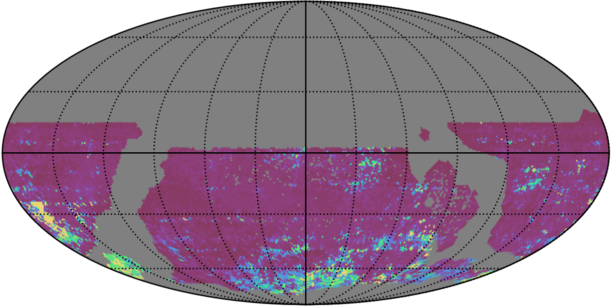
ddf_acor_sf25_lsf30_lsr10_v3.4_10yrs WFD i band: 75th Percentile Intranight Timespan
