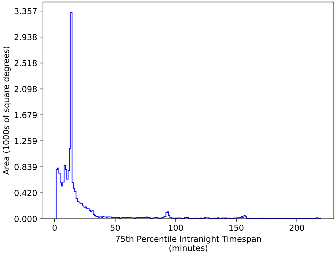
ddf_acor_sf25_lsf30_lsr10_v3.4_10yrs WFD i band: 75th Percentile Intranight Timespan
