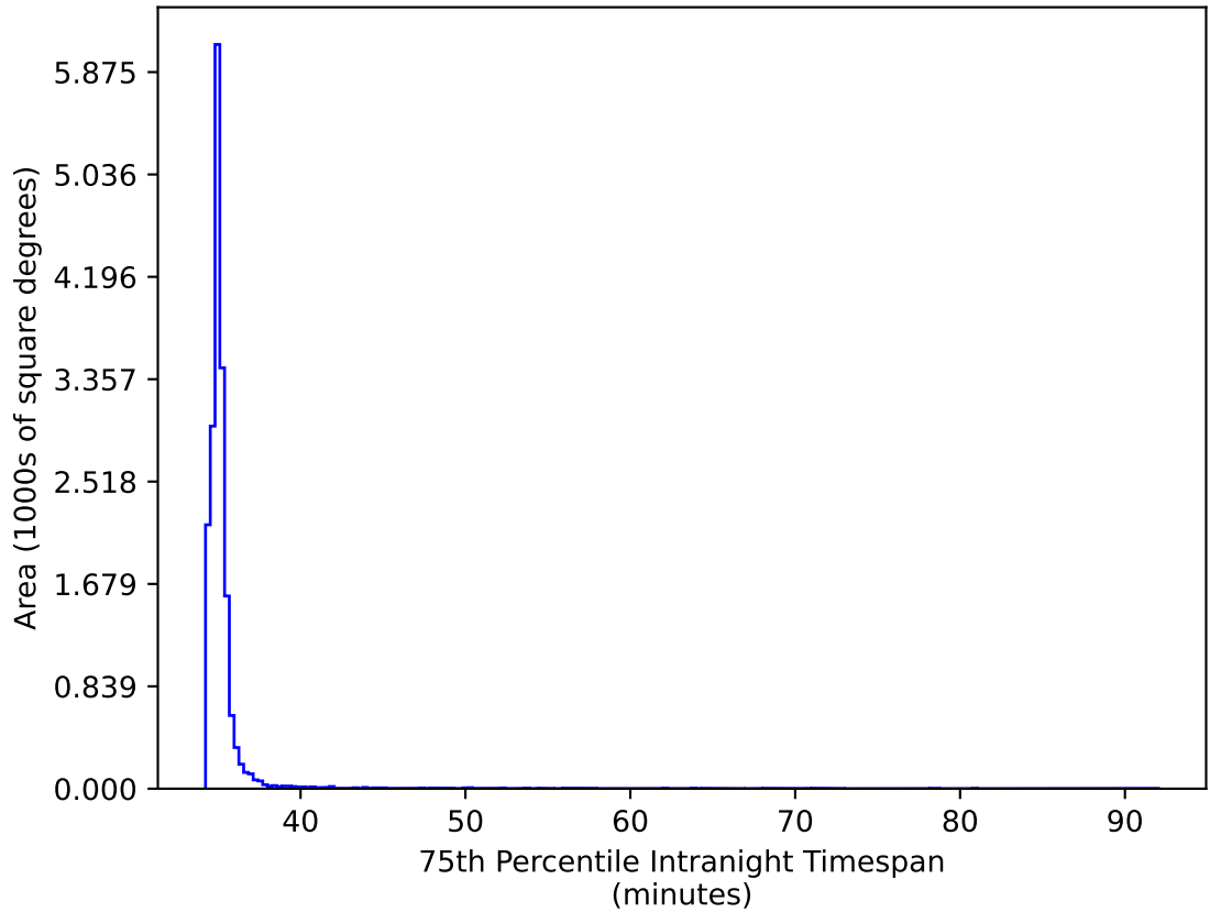
ddf_acor_sf25_lsf30_lsr10_v3.4_10yrs WFD gr bands: 75th Percentile Intranight Timespan
