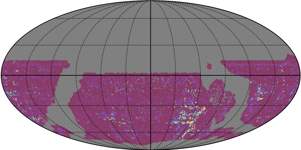
ddf_acor_sf25_lsf30_lsr10_v3.4_10yrs WFD g band: 75th Percentile Intranight Timespan
