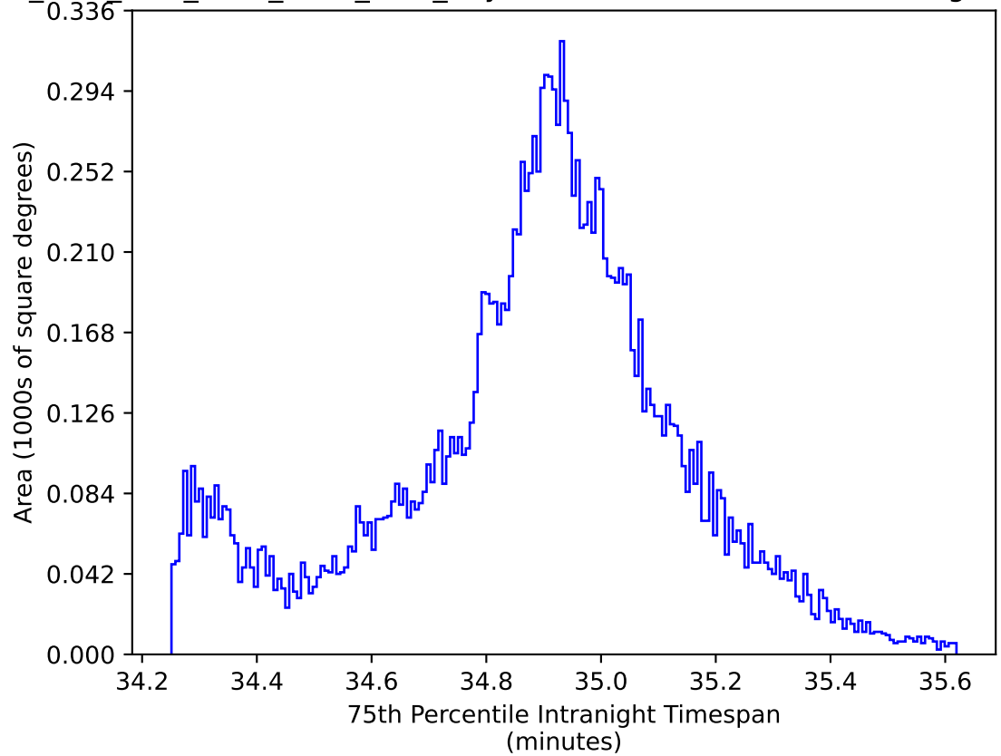
ddf_acor_sf25_lsf30_lsr10_v3.4_10yrs WFD: 75th Percentile Intranight Timespan
