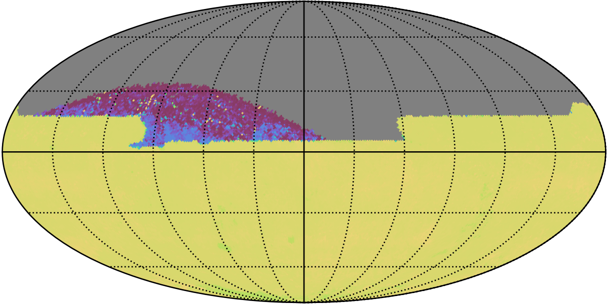
ddf_acor_sf25_lsf30_lsr10_v3.4_10yrs All sky zy bands: 75th Percentile Intranight Timespan
