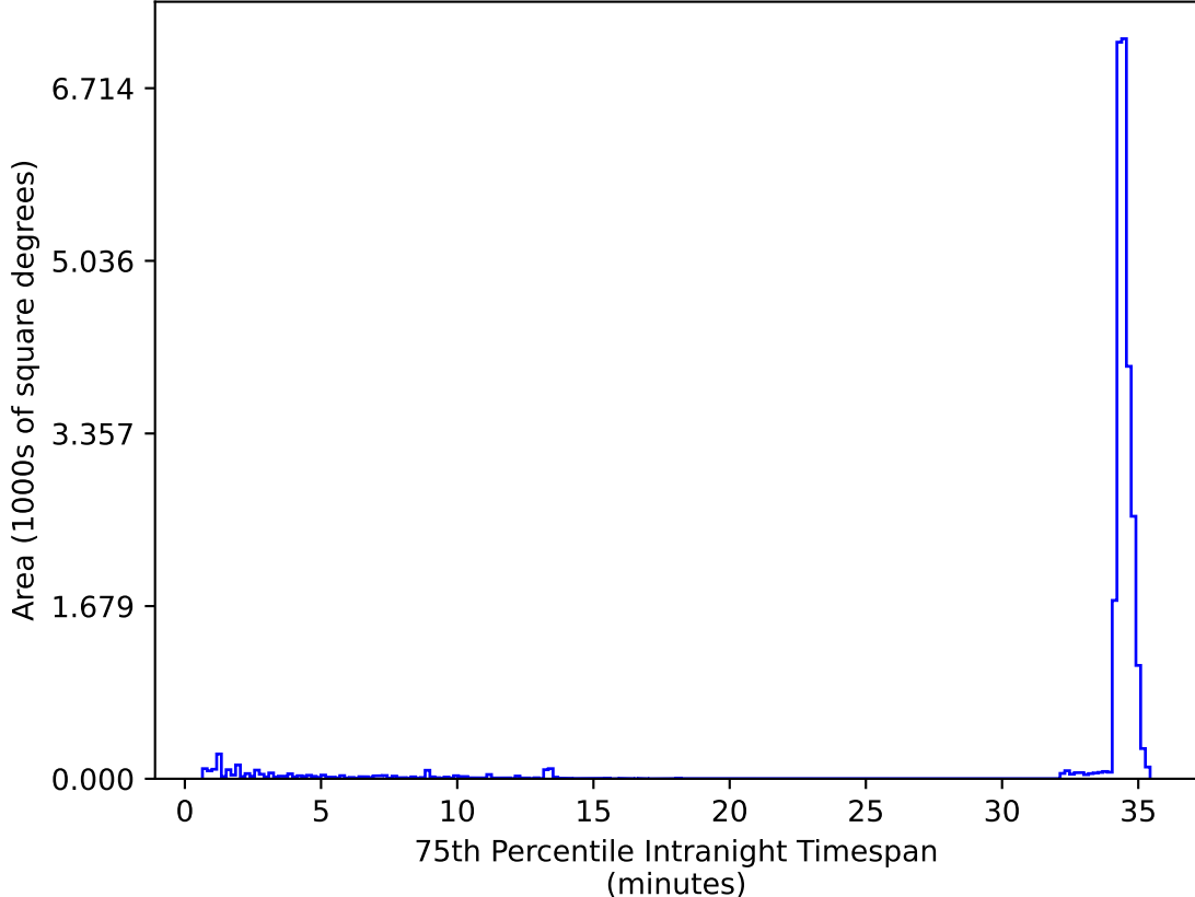
ddf_acor_sf25_lsf30_lsr10_v3.4_10yrs All sky zy bands: 75th Percentile Intranight Timespan
