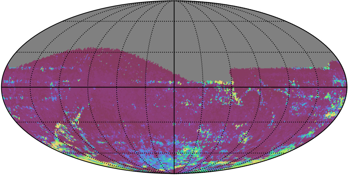
ddf_acor_sf25_lsf30_lsr10_v3.4_10yrs All sky z band: 75th Percentile Intranight Timespan
