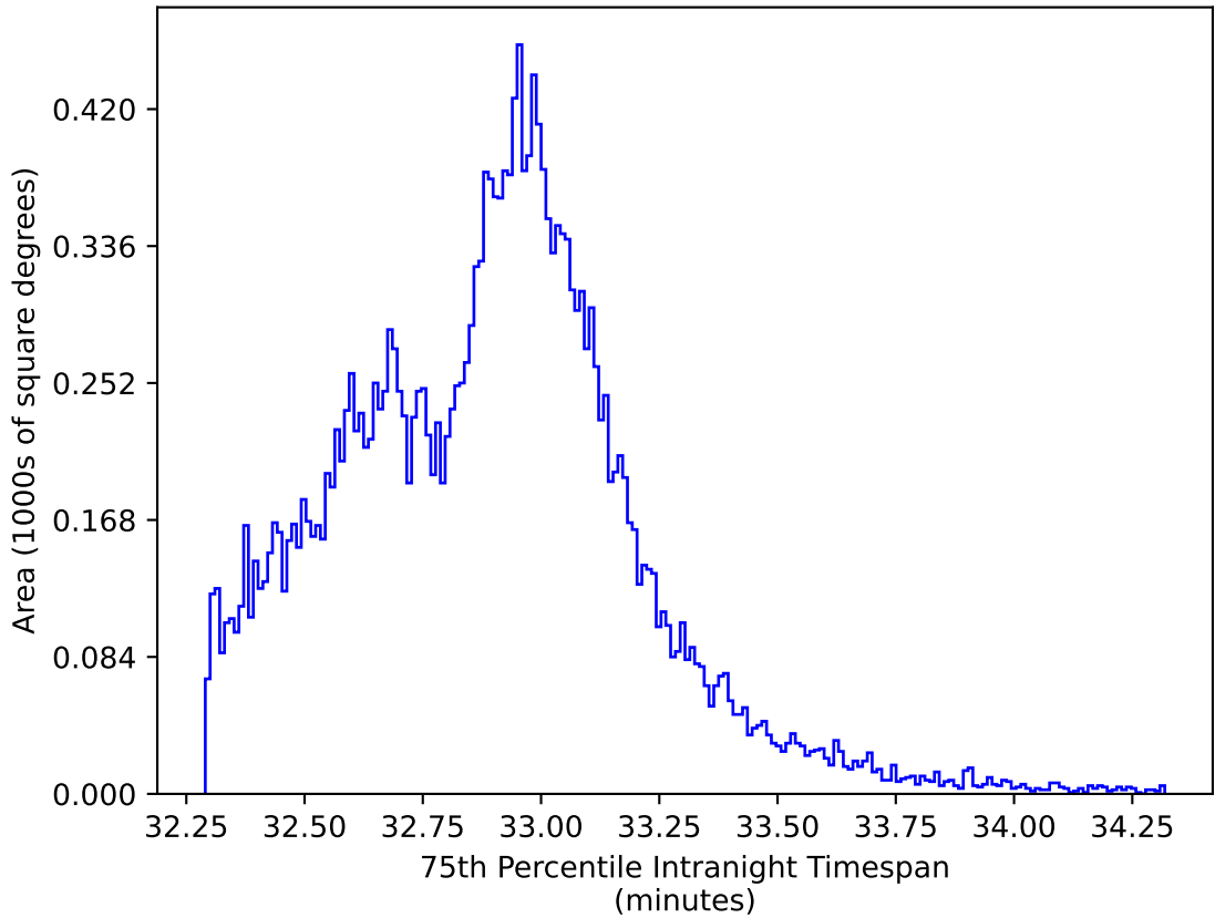
ddf_acor_sf25_lsf30_lsr10_v3.4_10yrs All sky y band: 75th Percentile Intranight Timespan
