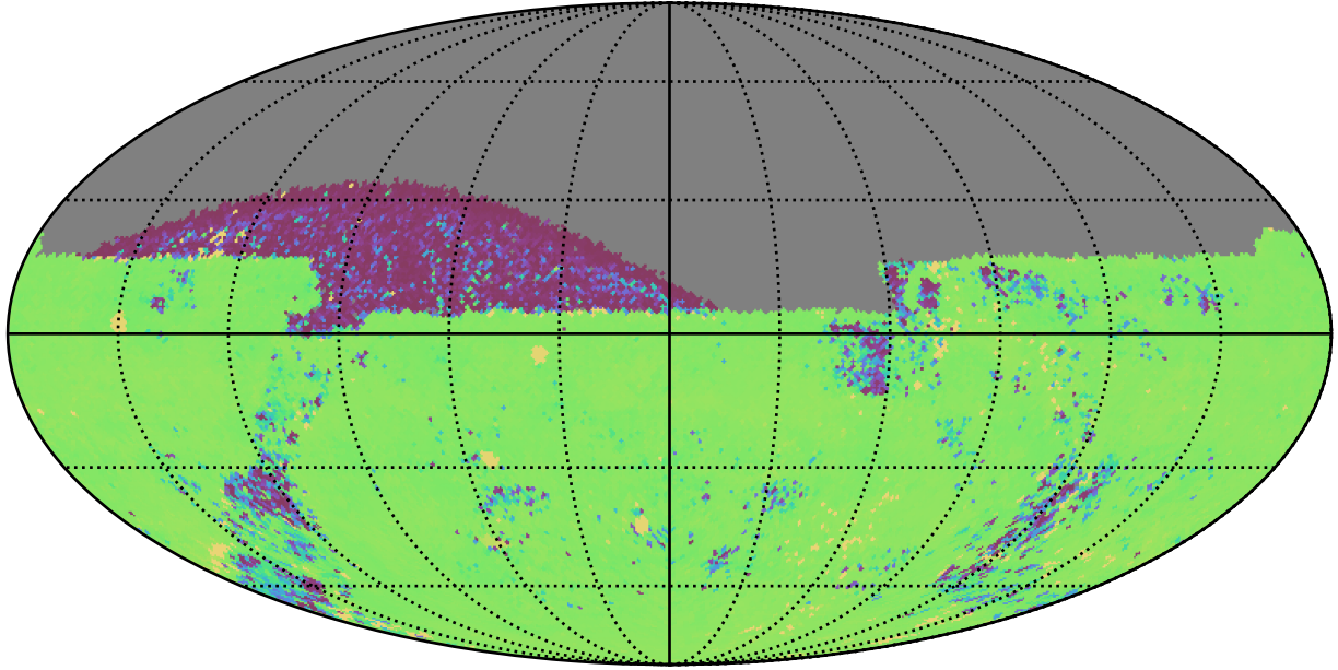
ddf_acor_sf25_lsf30_lsr10_v3.4_10yrs All sky ug bands: 75th Percentile Intranight Timespan
