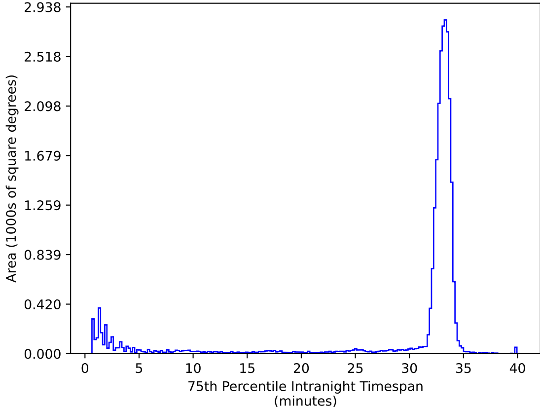
ddf_acor_sf25_lsf30_lsr10_v3.4_10yrs All sky ug bands: 75th Percentile Intranight Timespan
