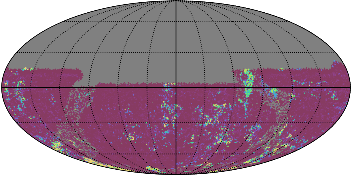
ddf_acor_sf25_lsf30_lsr10_v3.4_10yrs All sky u band: 75th Percentile Intranight Timespan
