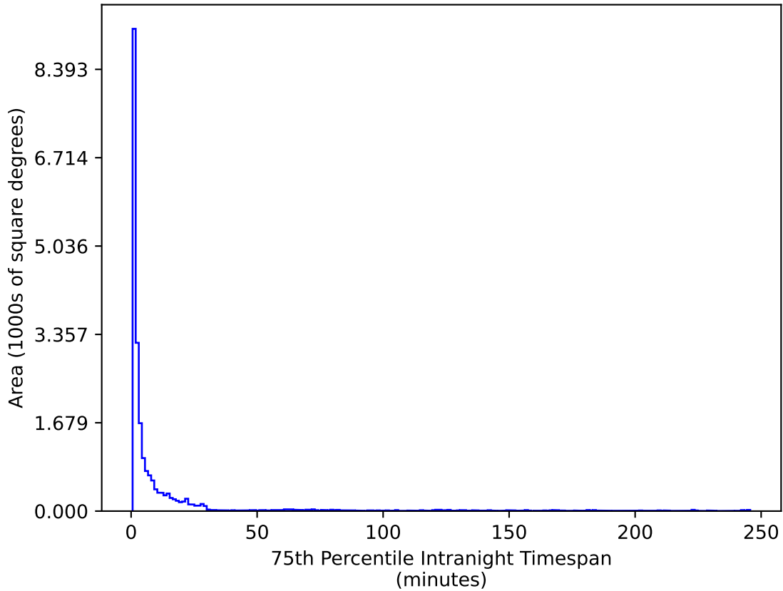
ddf_acor_sf25_lsf30_lsr10_v3.4_10yrs All sky u band: 75th Percentile Intranight Timespan
