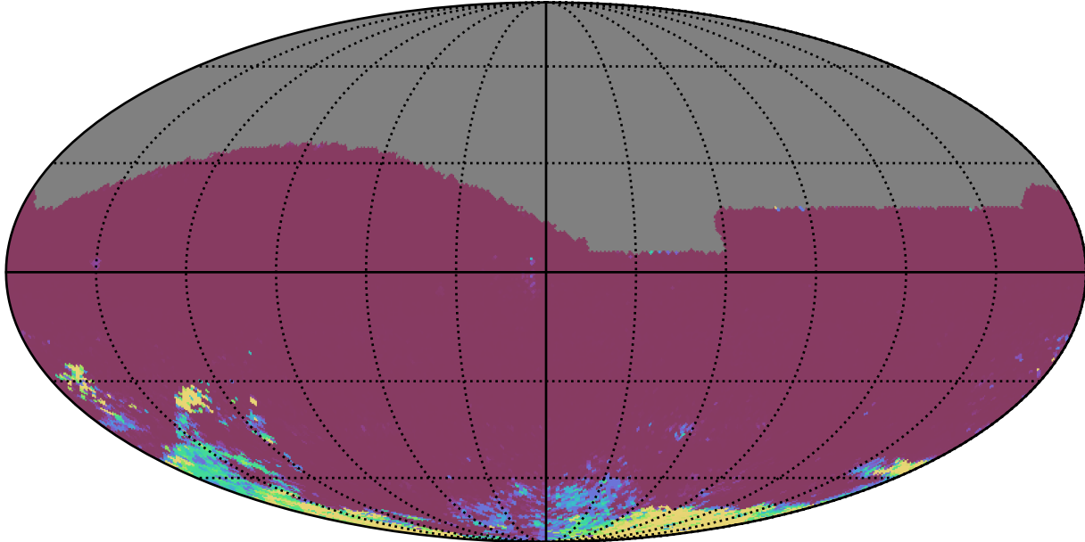
ddf_acor_sf25_lsf30_lsr10_v3.4_10yrs All sky ri bands: 75th Percentile Intranight Timespan
