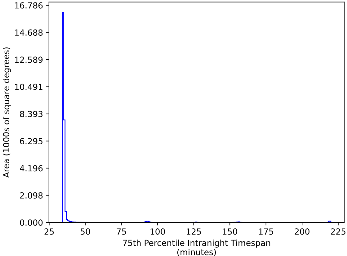
ddf_acor_sf25_lsf30_lsr10_v3.4_10yrs All sky ri bands: 75th Percentile Intranight Timespan
