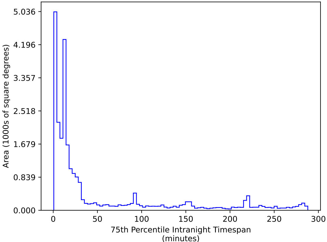
ddf_acor_sf25_lsf30_lsr10_v3.4_10yrs All sky r band: 75th Percentile Intranight Timespan
